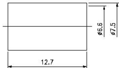
STRIPPING DIMENSION
