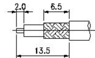
STRIPPING DIMENSION
